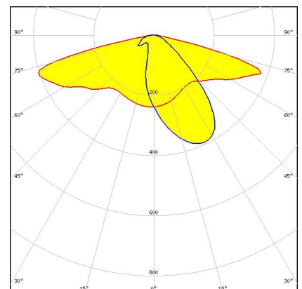
C12449_STRADA-T-6X1-DWC
