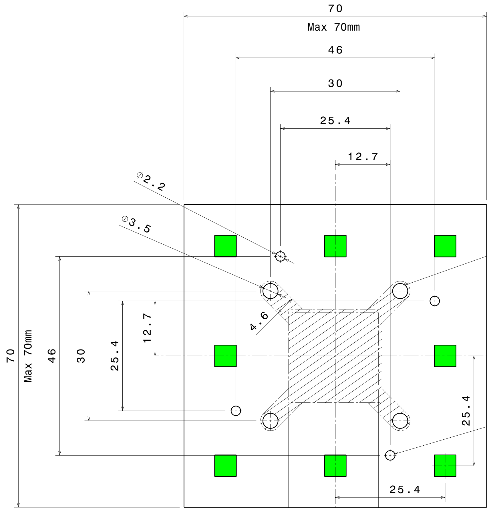
Front view Scale: 2:1
